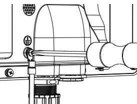
Figure 12: Attaching the Grounding Wire
