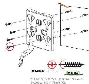
Figure 7: Attaching the Mounting Plate
