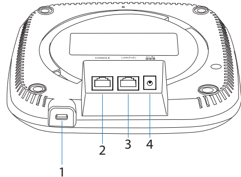
Figure 2: Rear Connectors
