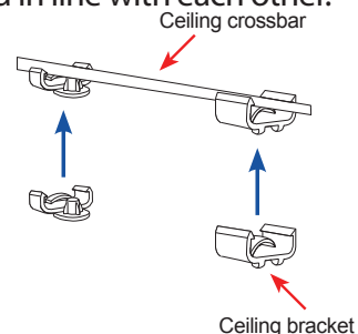
Figure 10: Attaching the Ceiling Brackets
