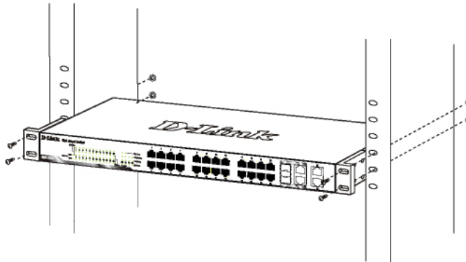
Mount the Switch in the rack
