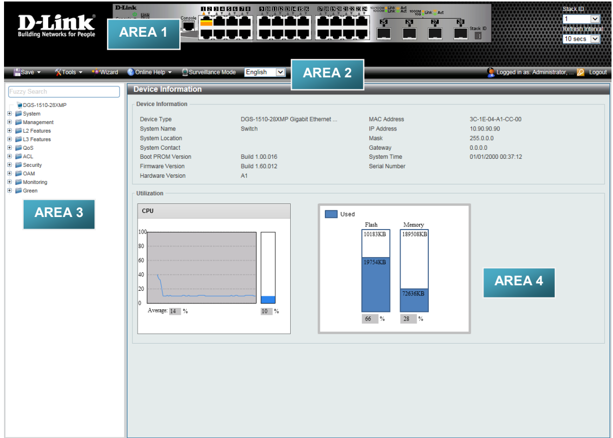
Figure 5-3 Web UI (Standard Mode)
