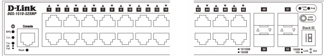
Figure 1-18 LED indicators for a DGS-1510-52XMP Switch
