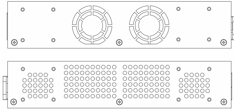
Figure 1-33 Side panels view of a DGS-1510-52 Switch
