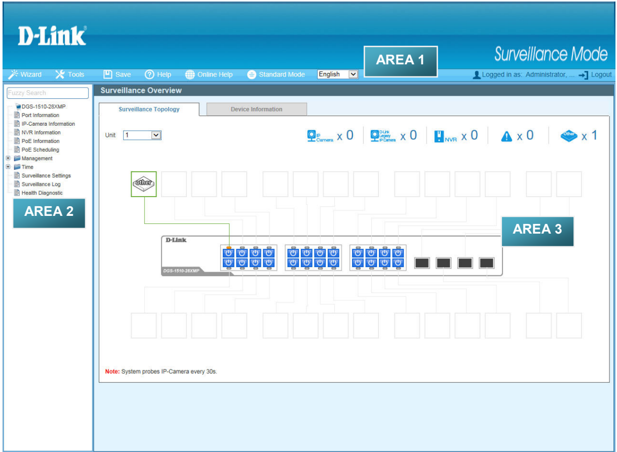
Figure 5-4 Web UI (Surveillance Mode)
