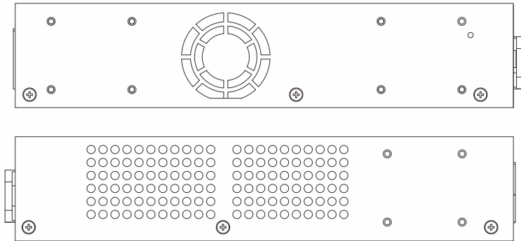
Figure 1-31 Side panels view of a DGS-1510-28X Switch
