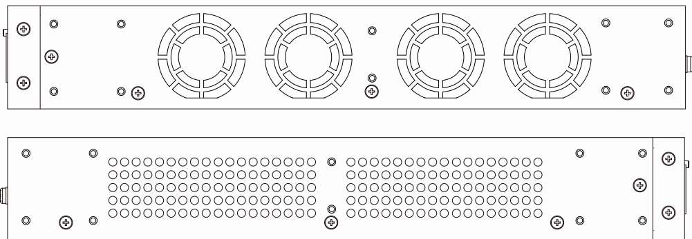
Figure 1-36 Side panels view of a DGS-1510-52XMP Switch
