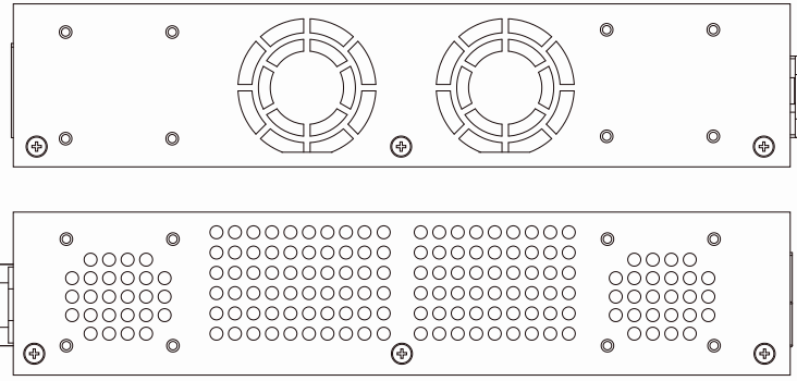
Figure 1-33 Side panels view of a DGS-1510-52 Switch
