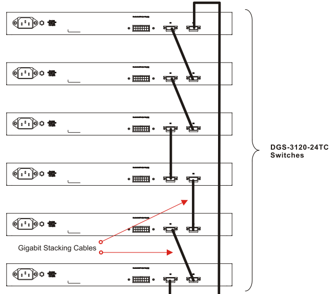
Figure 2-25 Switches stacked in a Duplex Ring
