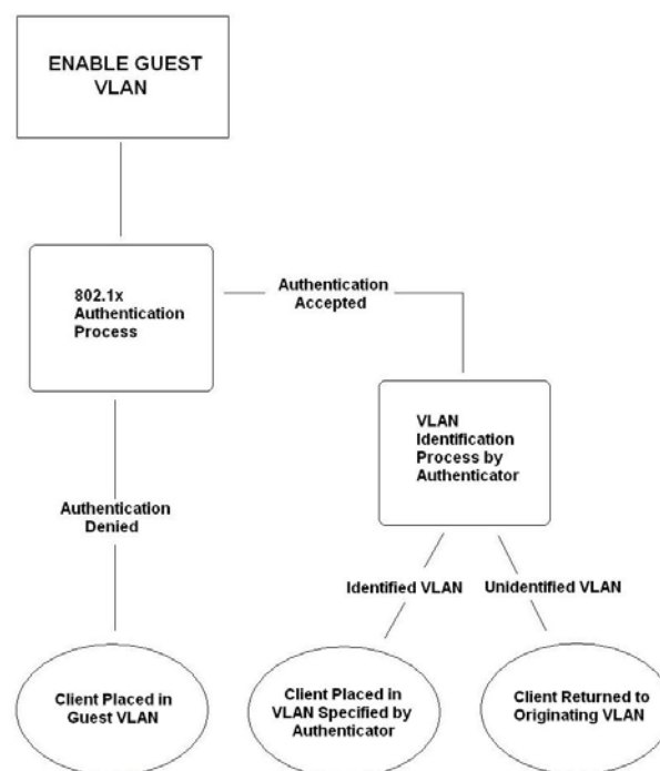
Figure 8-12 Guest VLAN Authentication Process
