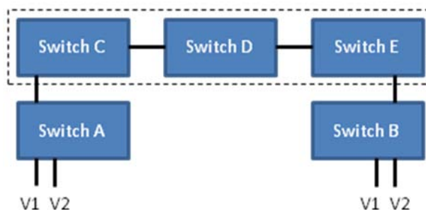
Figure 4-22 Example of VLAN Trunk
