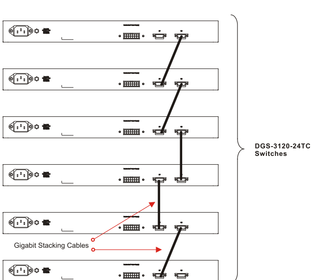
Figure 2-24 Switches stacked in a Duplex Chain
