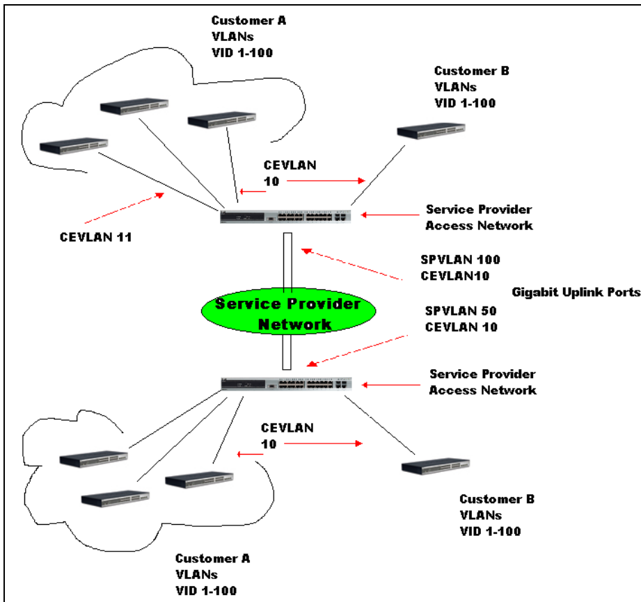
Figure 4-26 QinQ example window
