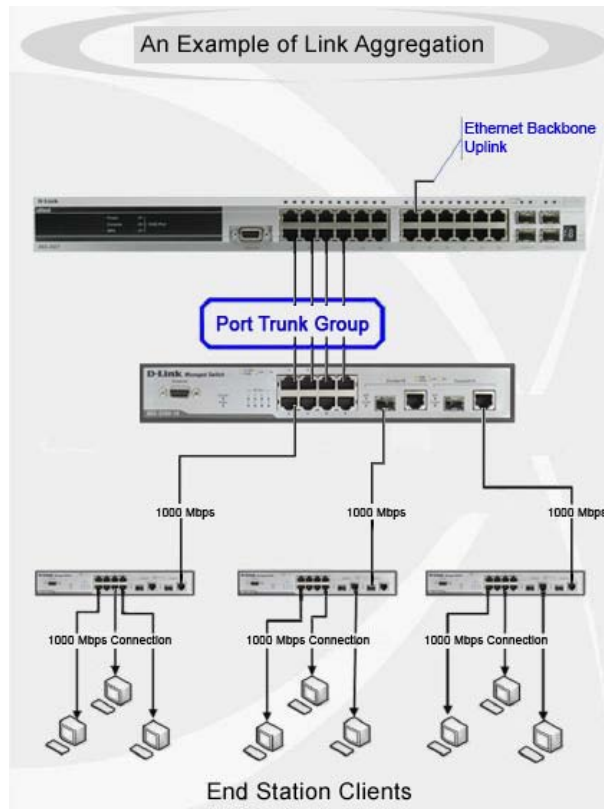
4-35 Example of Port Trunk Group
