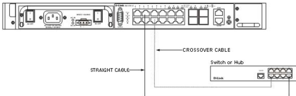
Figure 3- 2. The Switch connected to a normal (non-Uplink) port on a hub or switch using a straight or crossover cable
