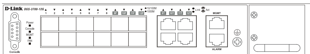
Figure 1- 4. LED Indicators on DGS-3700-12G switch
