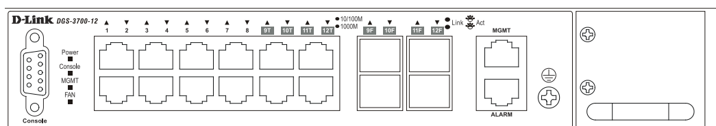
Figure 1- 3. LED Indicators on DGS-3700-12 switch
