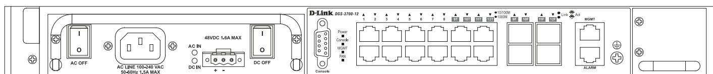
Figure 1- 1. Front Panel View of the DGS-3700-12 switch
