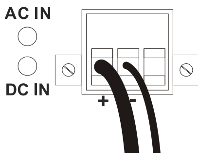
Figure 2- 6. Power connections attached to contacts after assembly
