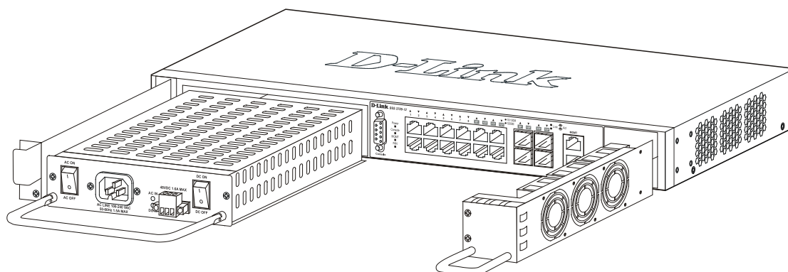
Figure 2- 5 Inserting/Removing the modules
