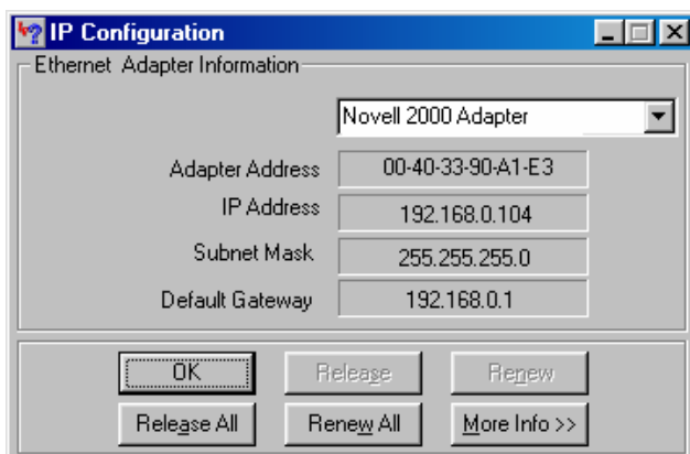
Figure 13: IP Configuration
