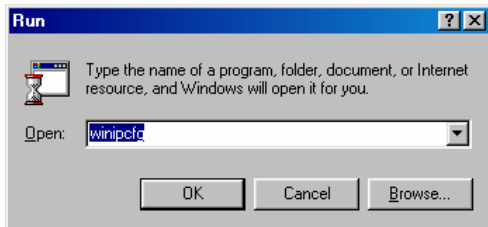
Figure 12: Run
