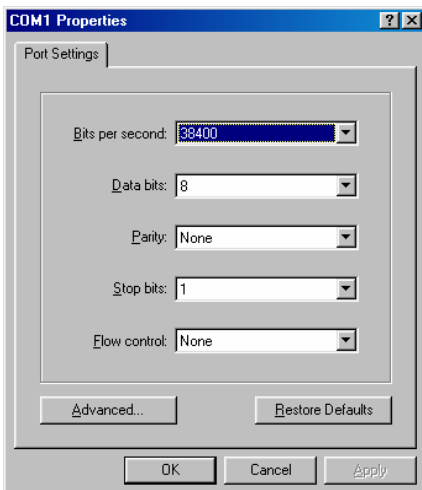
Figure 10: COM 1 Properties
