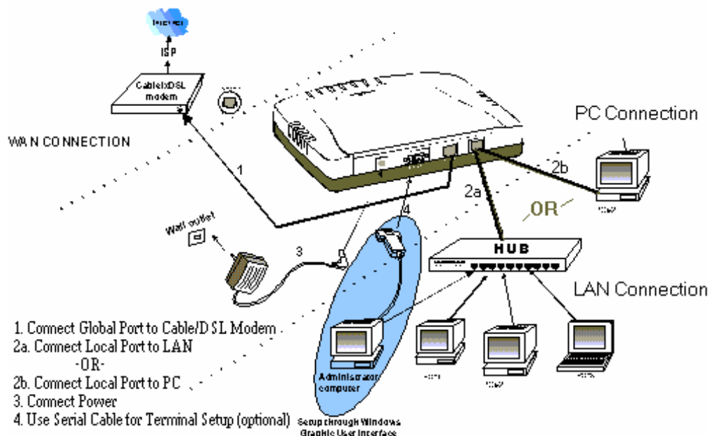
Figure 2: Hardware Connections
