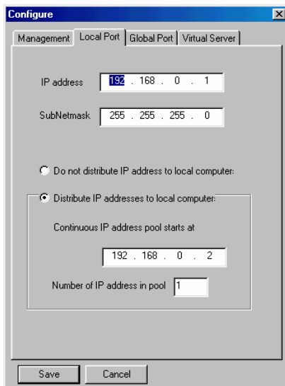
Figure 6: Local Port
