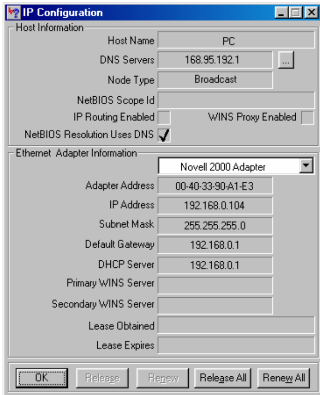
Figure 14: IP Configuration
