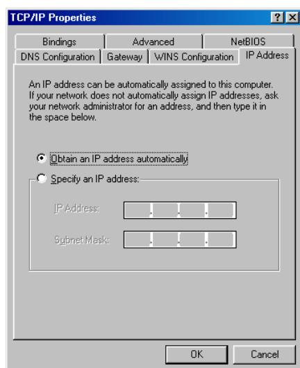
Figure 3: TCP/IP Properties
