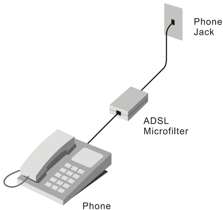
Microfilter Installation
