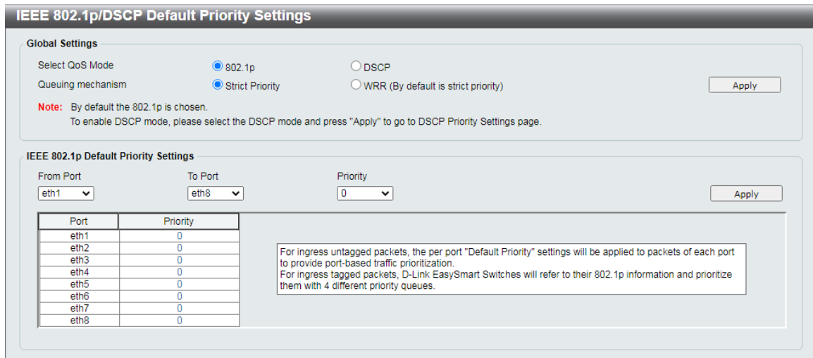
Figure 4.48 - QoS > 802.1p/DSCP Default Priority – 802.1p
