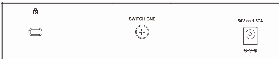
Figure 1.2 - DGS-1100-08PLV2 Rear Panel
