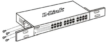
Figure 2. Attaching the mounting brackets
