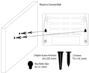
Figure 4. Mounting a desktop switch to a Wall
