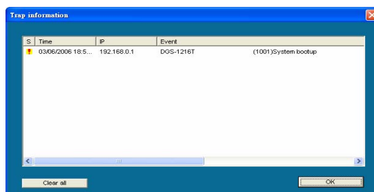
Figure 9 – Trap information
