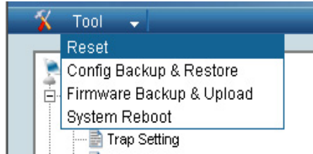
Figure 17 – Tool Menu
