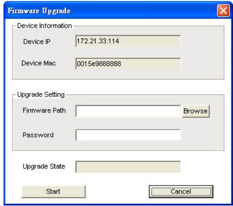
Figure 12 – Firmware Upgrade
