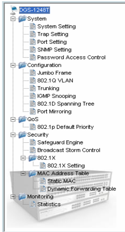
Figure 22 –Setup Menu
