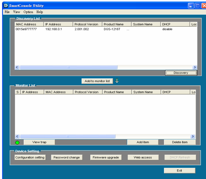
Figure 7 – SmartConsole Utility
