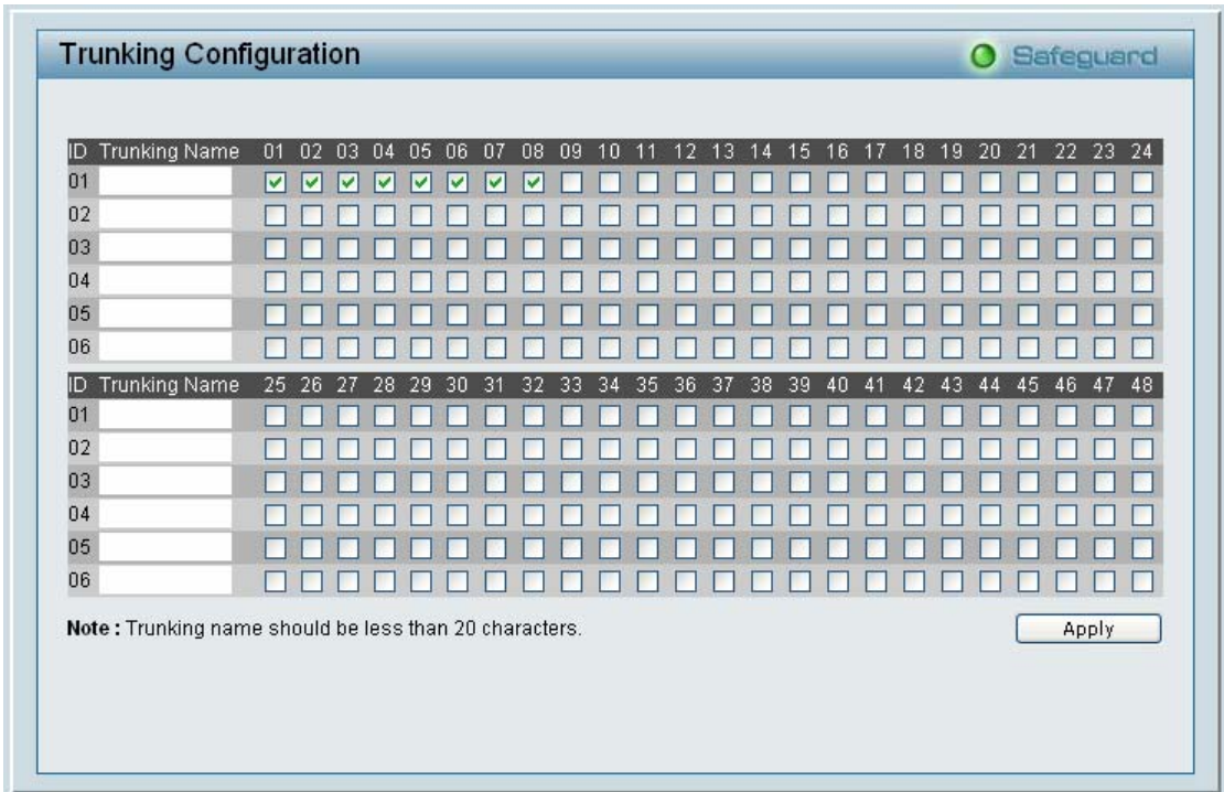
Figure 32 – Configuration > Trunking
