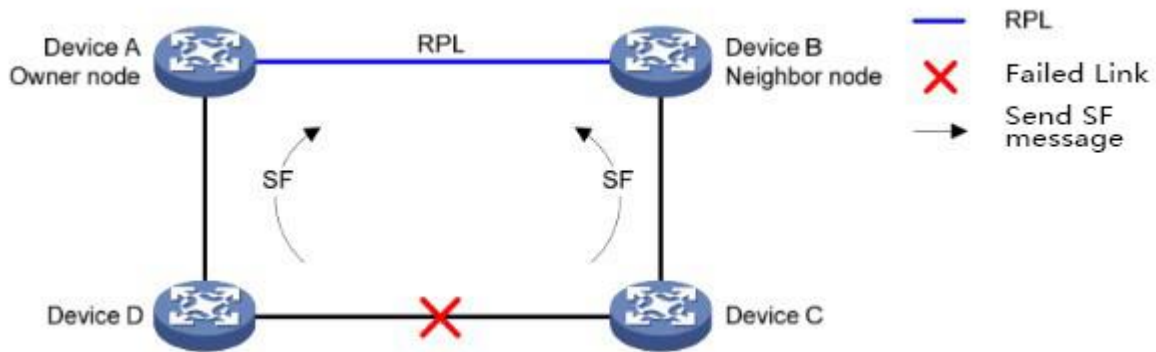
Figure2 ERPS Link interruption protection switching
