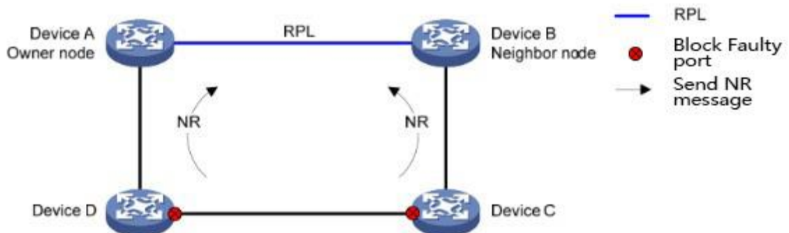
Figure2 ERPS Link recovery and switchback
