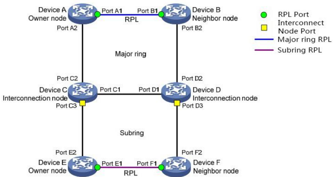
Figure 1 ERPS network diagram
