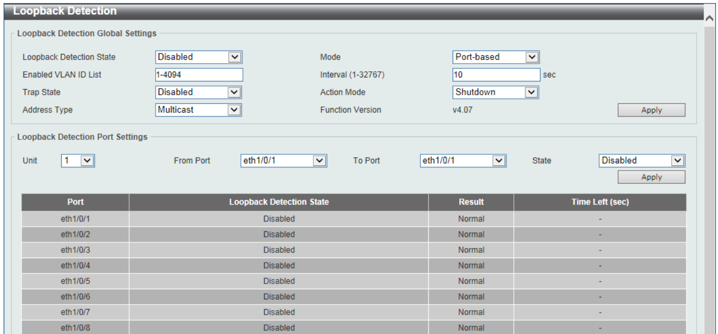
Figure 5-59 Loopback Detection Window
