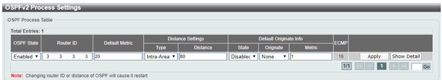
Figure 6-36 OSPFv2 Process Settings (Edit) Window
