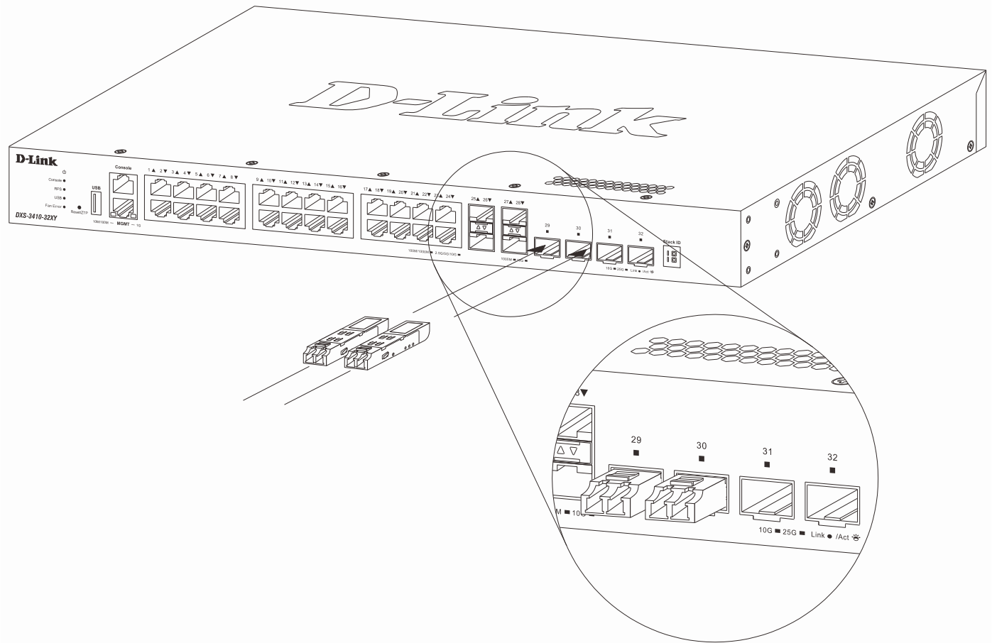
Figure 3-4 Inserting SFP28 transceivers into the SFP28 ports
