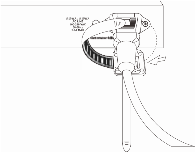
Figure 3-8 Circle around the power cord
