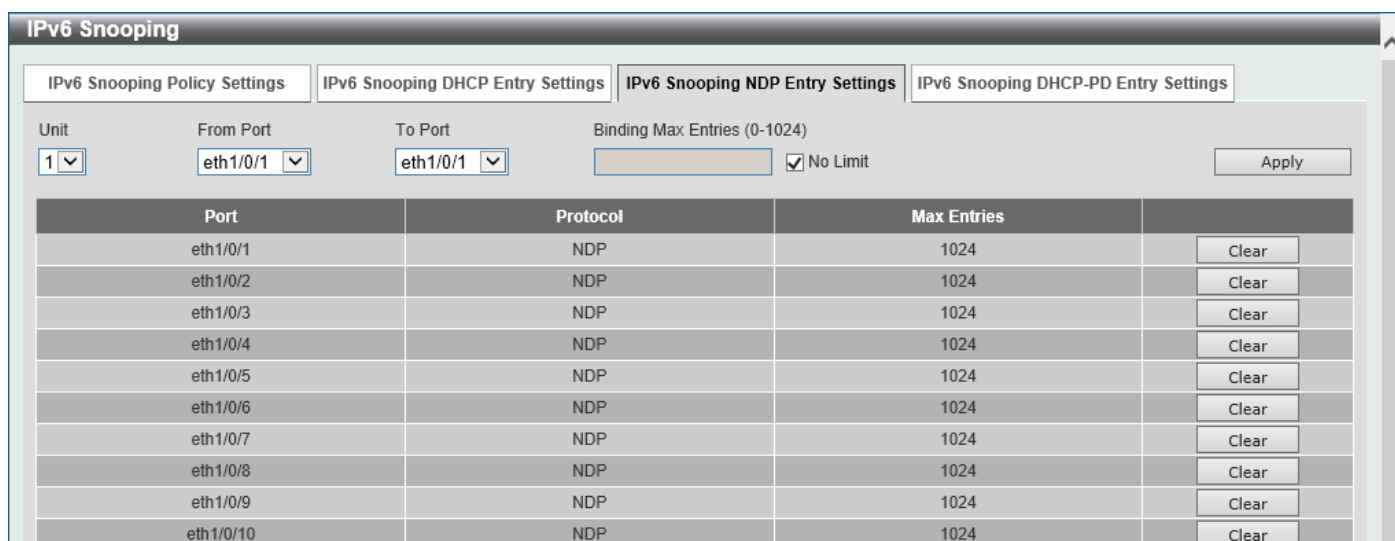
Figure 9-588 IPv6 Snooping (IPv6 Snooping NDP Entry Settings) Window
