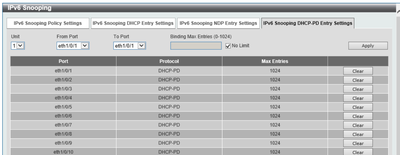
Figure 9-59 IPv6 Snooping (IPv6 Snooping DHCP-PD Entry Settings) Window
