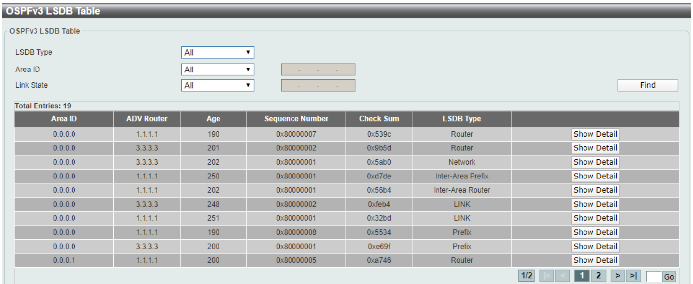
Figure 6-65 OSPFv3 LSDB Table Window
