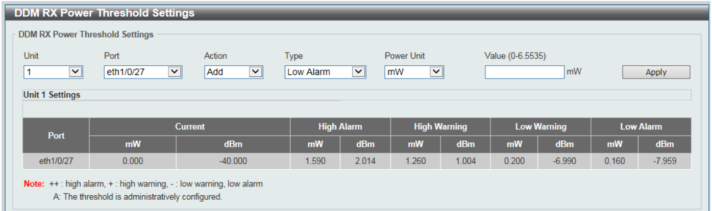
Figure 10-282 DDM RX Power Threshold Settings Window
