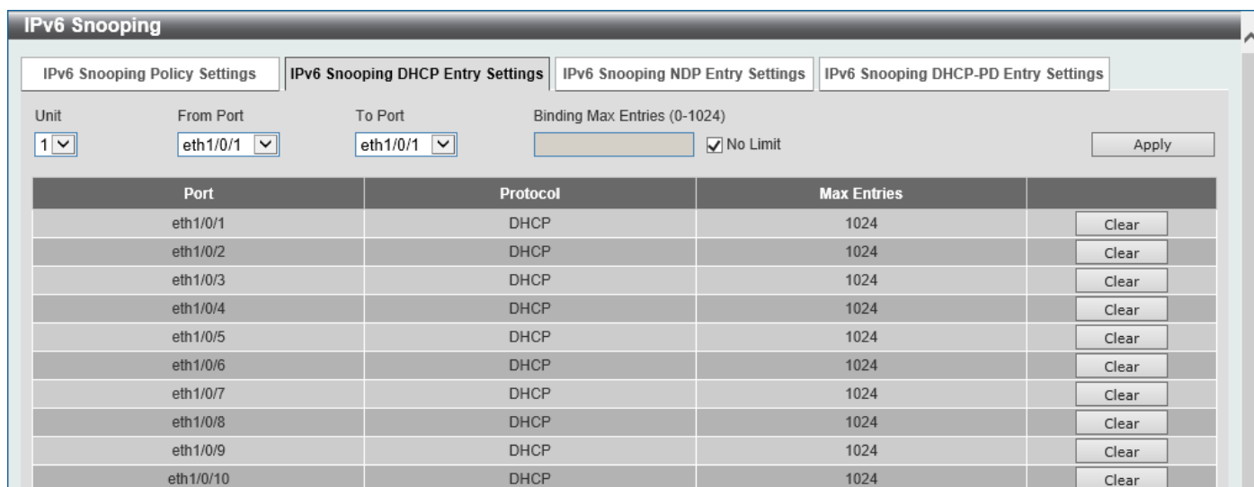
Figure 9-577 IPv6 Snooping (IPv6 Snooping DHCP Entry Settings) Window
