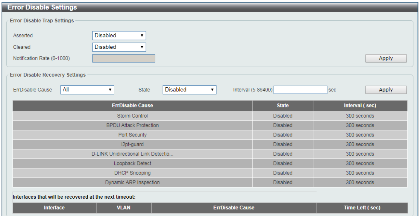
Figure 3-8 Error Disable Settings Window
