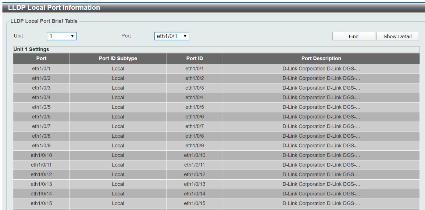
Figure 5-92 LLDP Local Port Information Window
