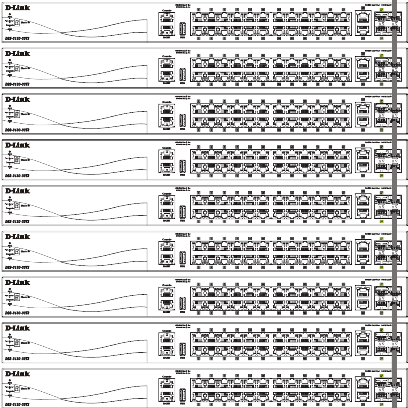
Figure 4-69 Duplex Ring stacking topology (SFP+)
