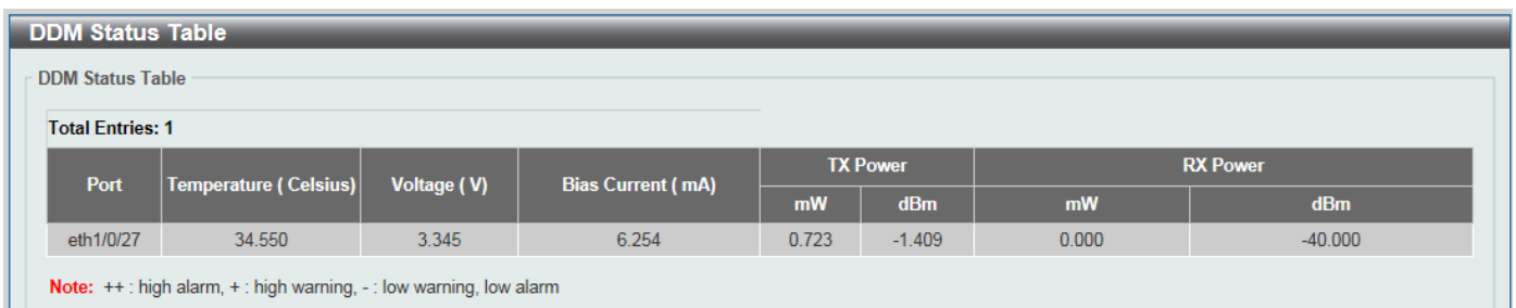
Figure 10-293 DDM Status Table Window
