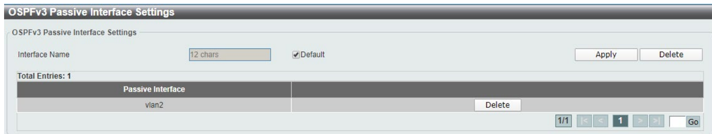
Figure 6-56 OSPFv3 Passive Interface Settings Window
