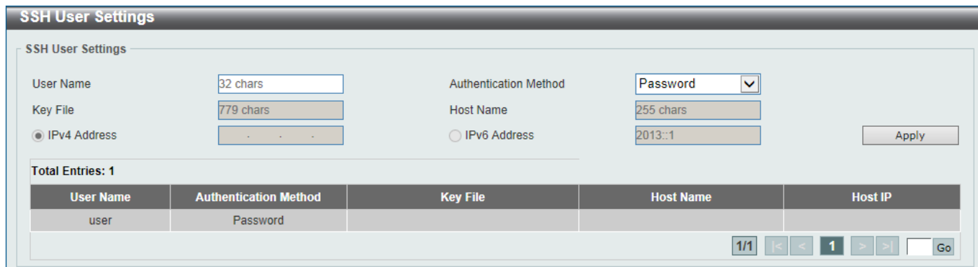
Figure 9-825 SSH User Settings Window
