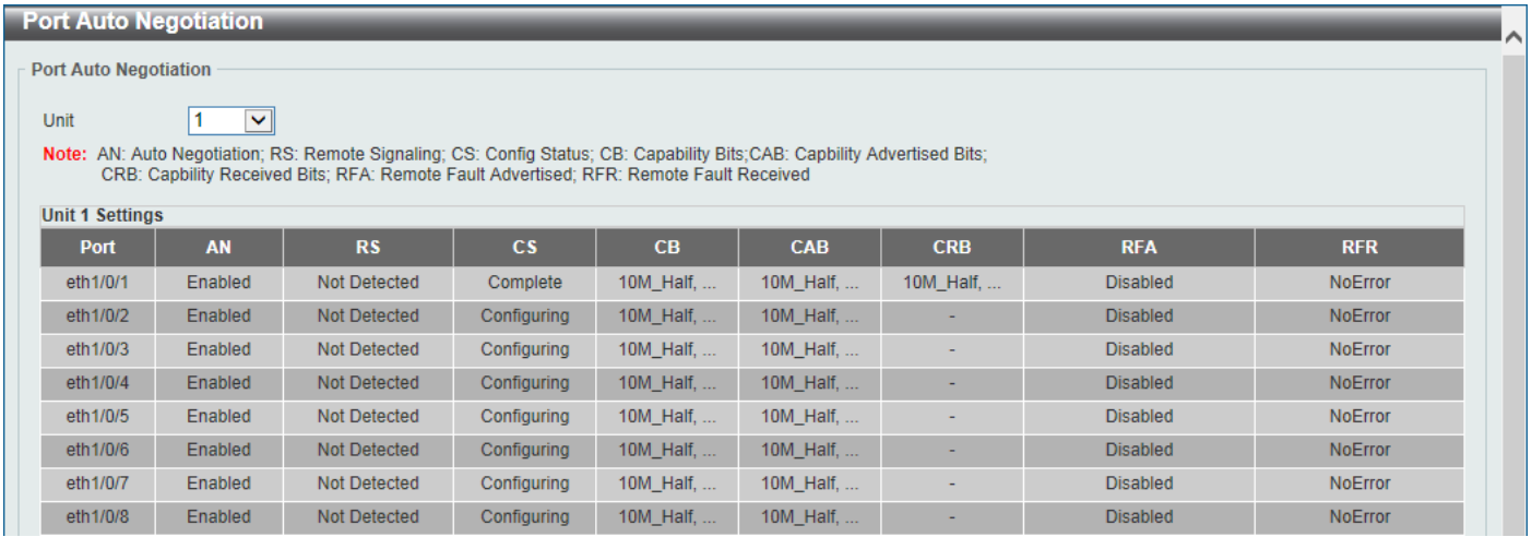
Figure 3-7 Port Auto Negotiation Window
