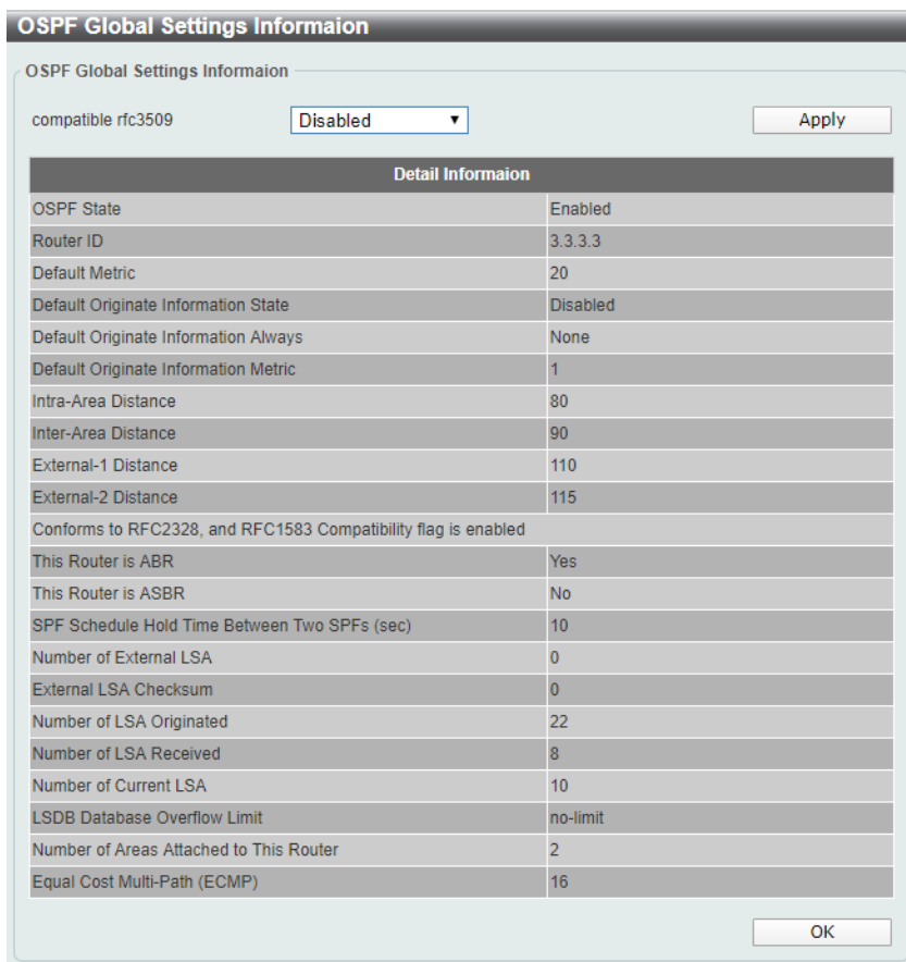
Figure 6-37 OSPFv2 Process Settings (Show Detail) Window
