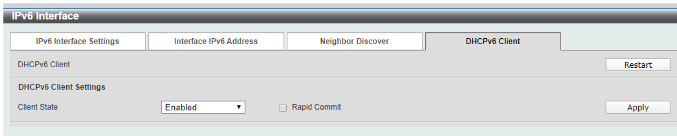
Figure 6-65 IPv6 Interface (Detail, DHCPv6 Client) Window
