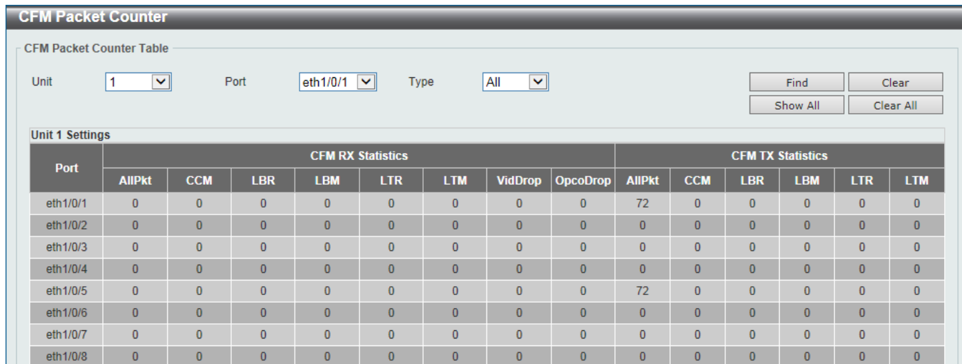
Figure 10-17 CFM Packet Counter Window
