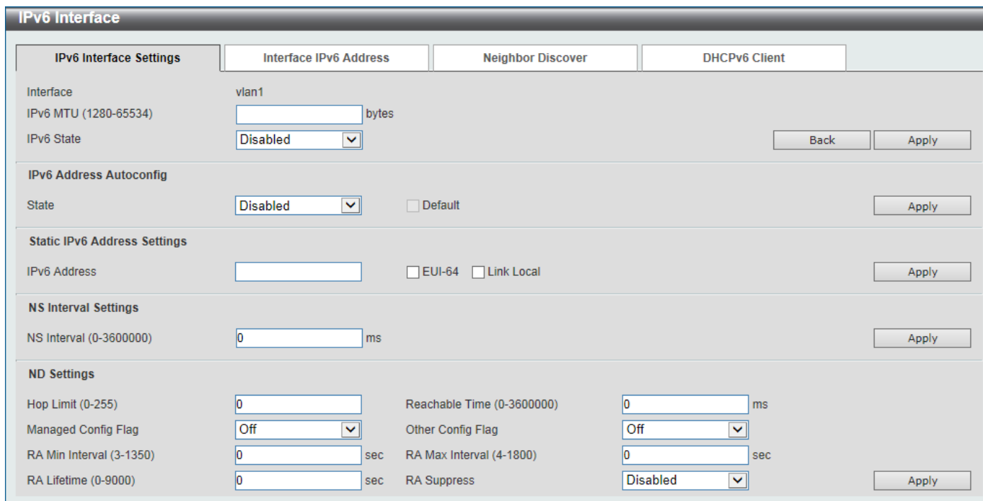
Figure 6-32 IPv6 Interface (Detail, IPv6 Interface Settings) Window
