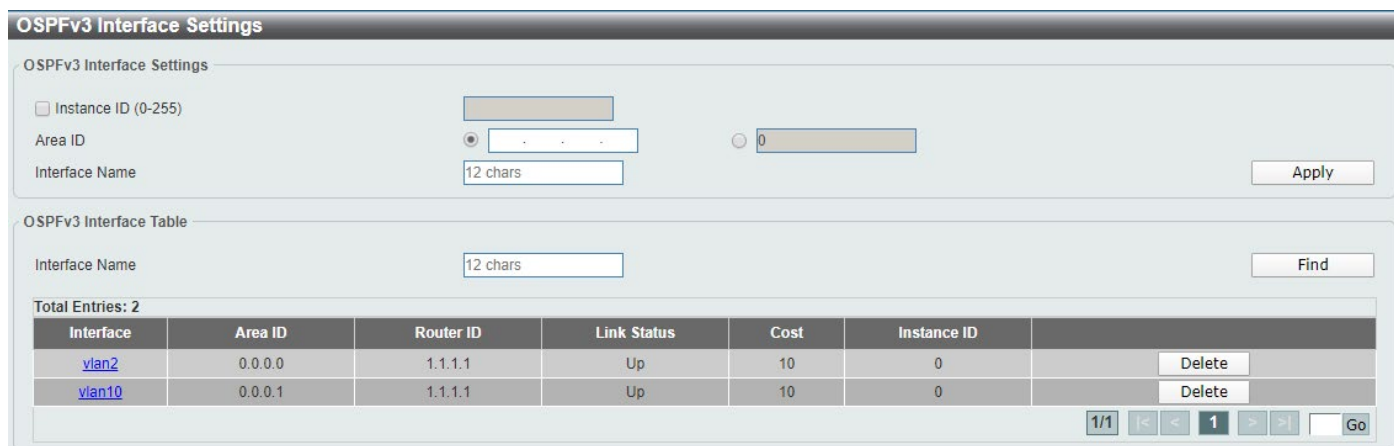
Figure 6-60 OSPFv3 Interface Settings Window
