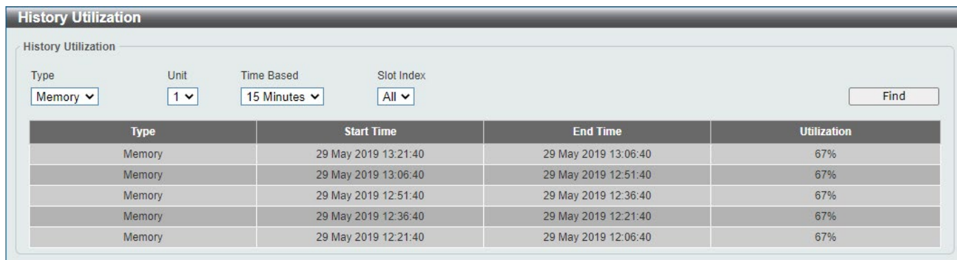
Figure 11-2 History Utilization (Memory) Window
