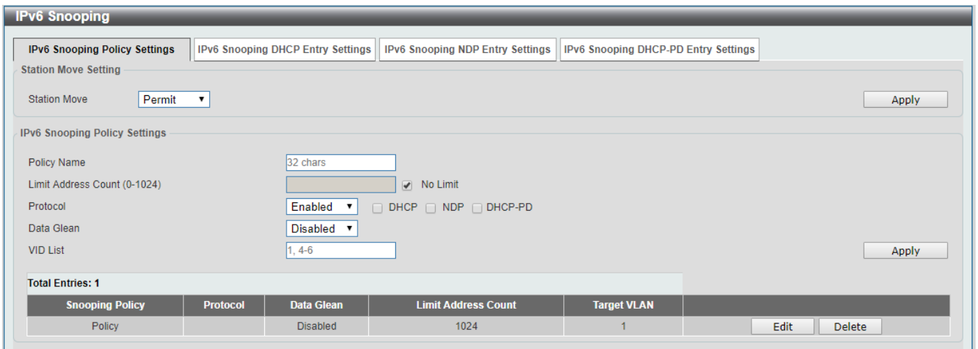
Figure 9-56 IPv6 Snooping Window
