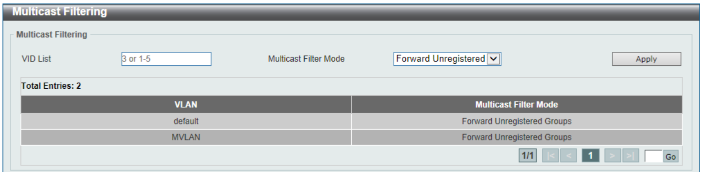
Figure 5-83 Multicast Filtering Window
