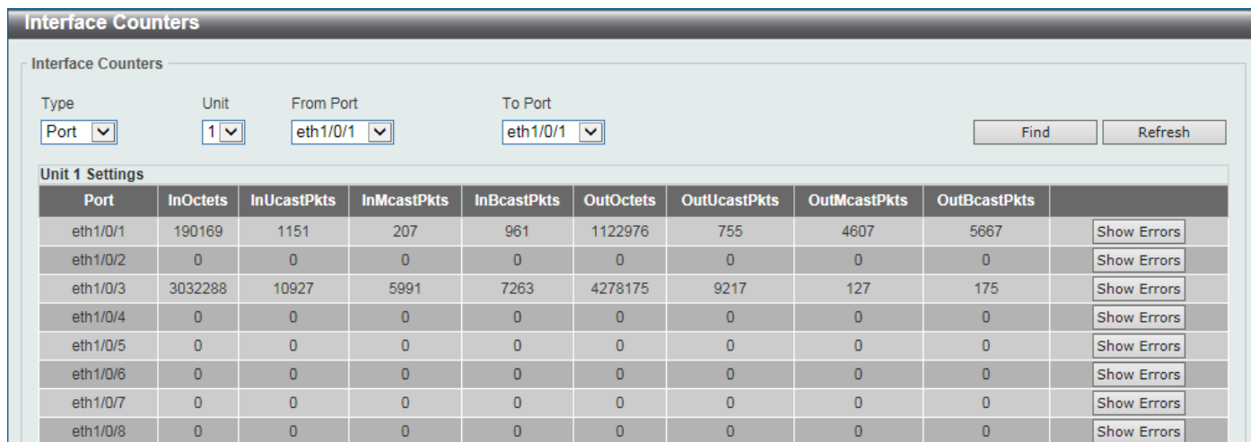
Figure 11-9 Interface Counters (Port) Window
