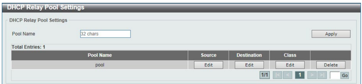
Figure 4-456 DHCP Relay Pool Settings Window
