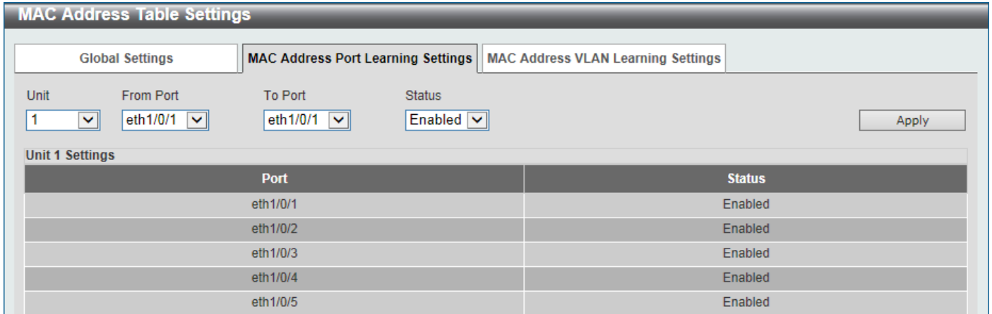
Figure 5-4 MAC Address Table Settings (MAC Address Port Learning Settings) Window
