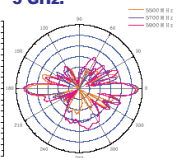
V-plane Co-polarization Pattern
