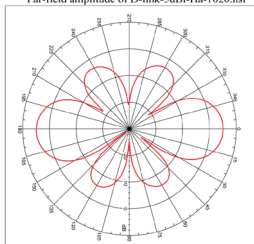
Far-field amplitude of D-link-5dBi-Ha-1020.nsi
