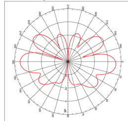
Far-field amplitude of D-link-7dBi-v1-1020.msi
