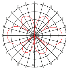
Far-field amplitude of D-link-5dBi-v-1020.nsi
