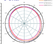
V-plane Co-polarization Pattern
