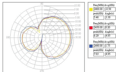
Test Mode: H Plane
