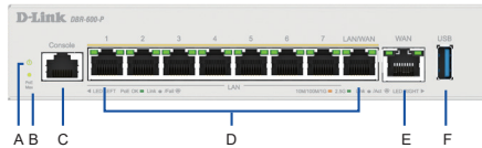
Figure 1. DBR-600-P Front Panel
