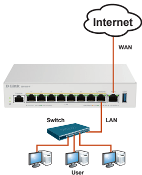
Figure 3. Basic Cabling Example
