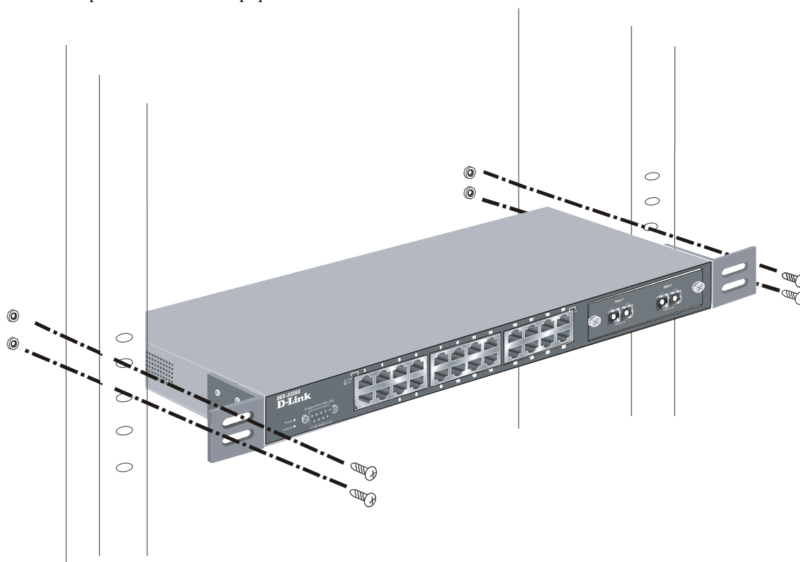
Figure 2-3. Installing the Switch on an equipment rack
