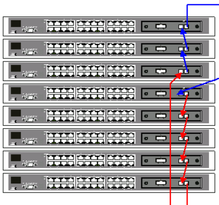
Figure 4 - 2. Switch Stack connections between optional stacking modules
