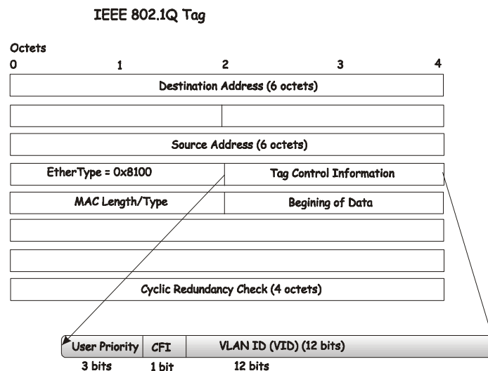
Figure 5 - 5. IEEE 802.1Q Tag
