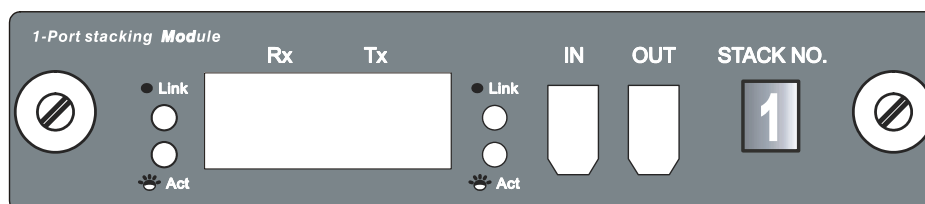
Figure 6 - 11. The Stacking Module's Front Panel
