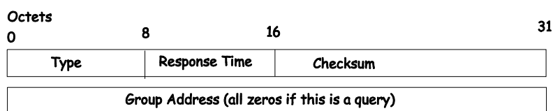
Figure 5 - 8. IGMP Message Format
