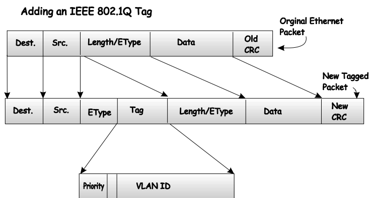
Figure 5 - 6. Adding an IEEE 802.1Q Tag
