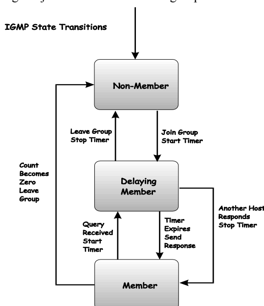
Figure 5 - 9. IGMP State Transitions
