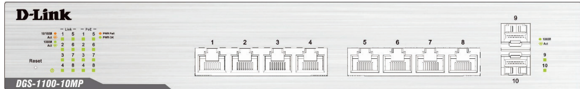
Figure 2-1 - DGS-1100-10MP Front Panel
