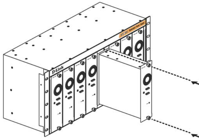
Figure 2 - 6. Installing the DPS-200 into the DPS-900
