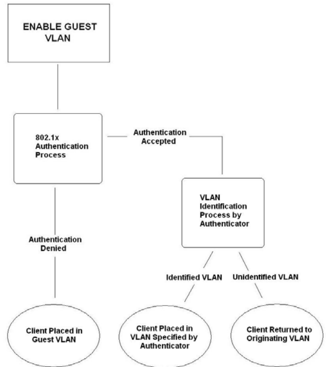
Figure 11- 17. Guest VLAN Authentication Process
