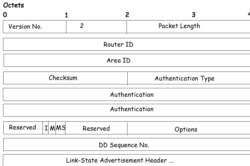
Figure 8- 33. Database Description Packet
