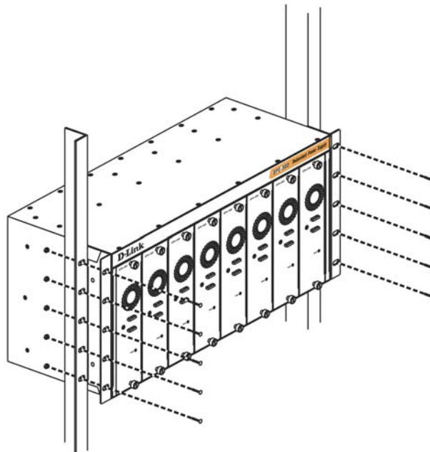
Figure 2 - 7. Installing the DPS-900 into the equipment rack
