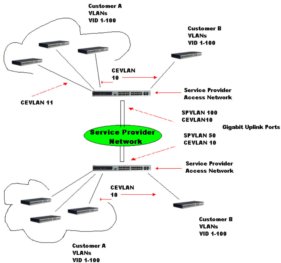
Figure 7- 8. Double VLAN Example
