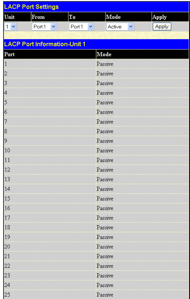
Figure 7- 22. LACP Port Settings window
