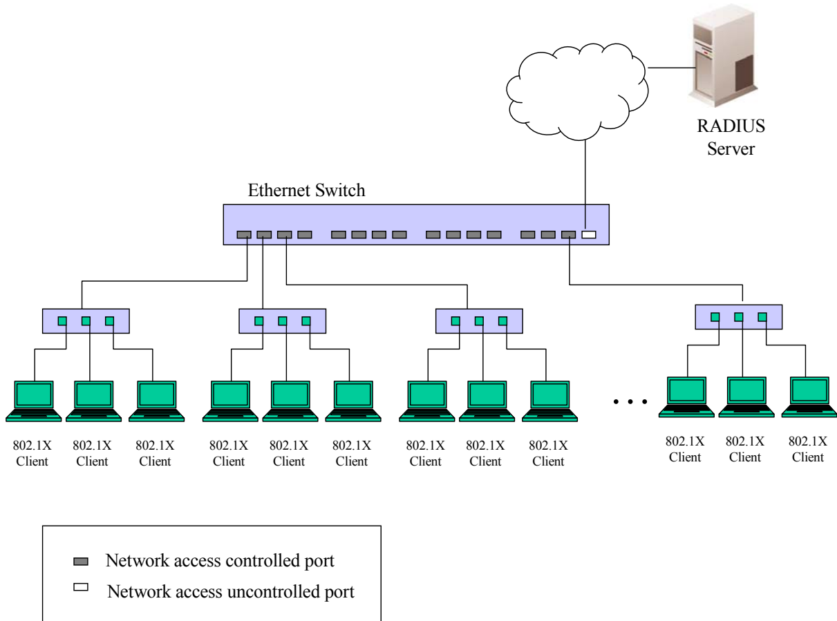
Figure 11- 16. Example of Typical MAC-Based Configuration
