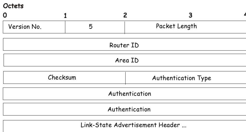
Figure 8- 36. Link State Acknowledge Packet
