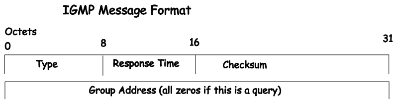
Figure 8- 78. IGMP Message Format
