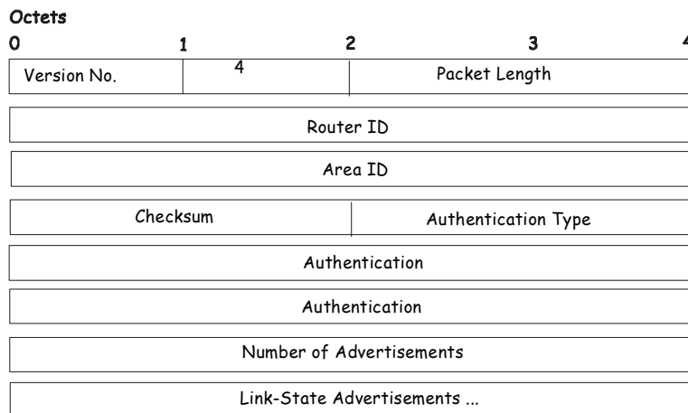
Figure 8- 35. Link-State Update Packet
