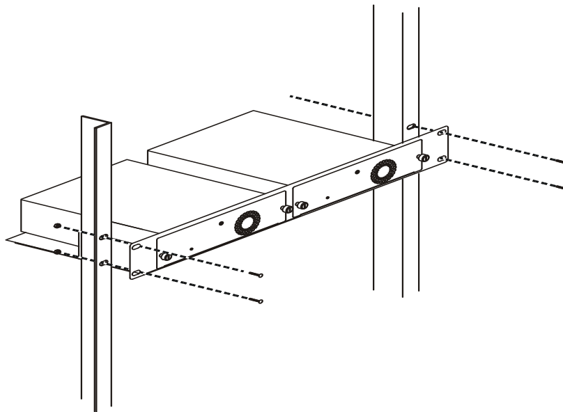
Figure 2 - 9. Install DPS-800 in an Equipment Rack
