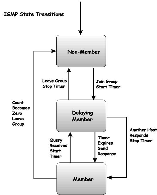
Figure 8- 79. IGMP State Transitions
