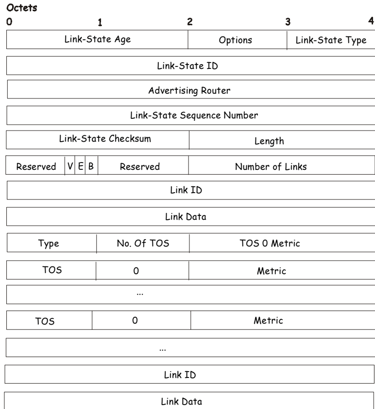
Figure 8- 38. Routers Links Advertisements
