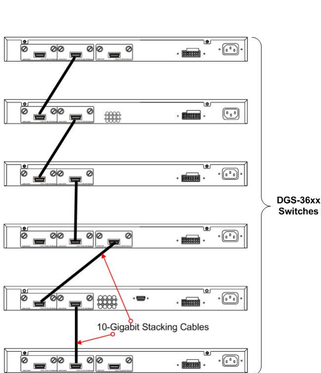
Figure 6- 4. Switches stacked in a Duplex Chain
