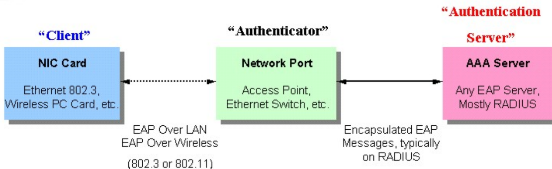
Figure 11- 10. The three roles of 802.1X
