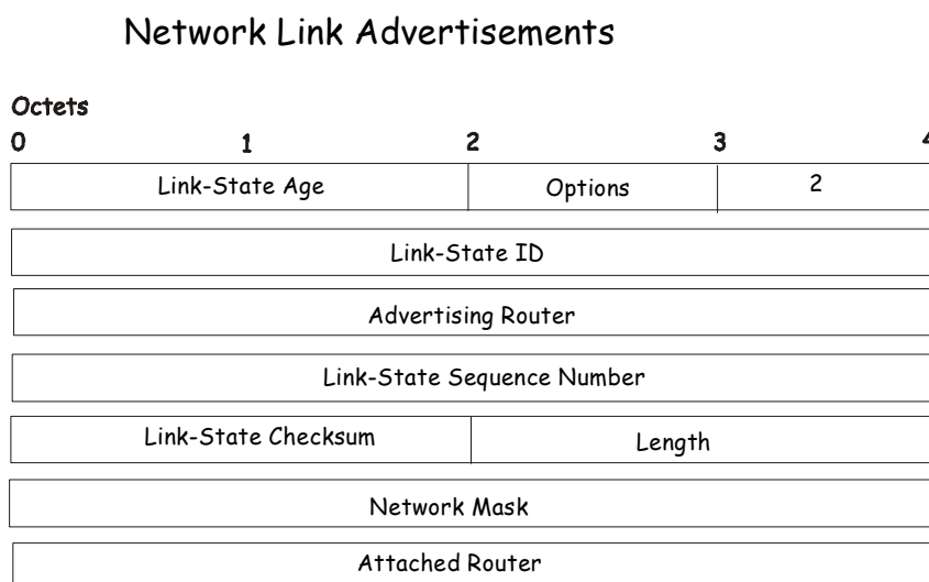
Figure 8- 39. Network Link Advertisements
