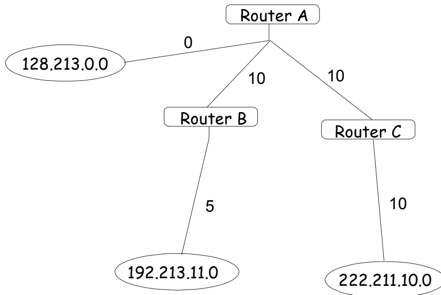
Figure 8- 30. Constructing a Shortest Path Tree - Completed
