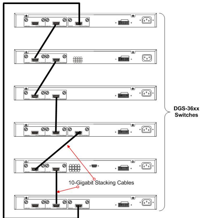
Figure 6- 5. Switches stacked in a Duplex Ring
