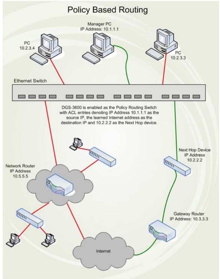
Figure 8- 21. Policy-based Routing example
