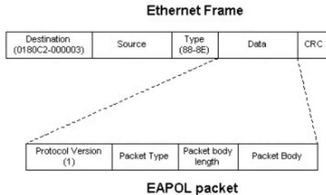
Figure 11- 9. The EAPOL Packet
