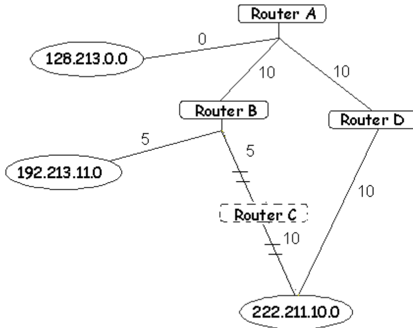
Figure 8- 28. Constructing a Shortest Path Tree
