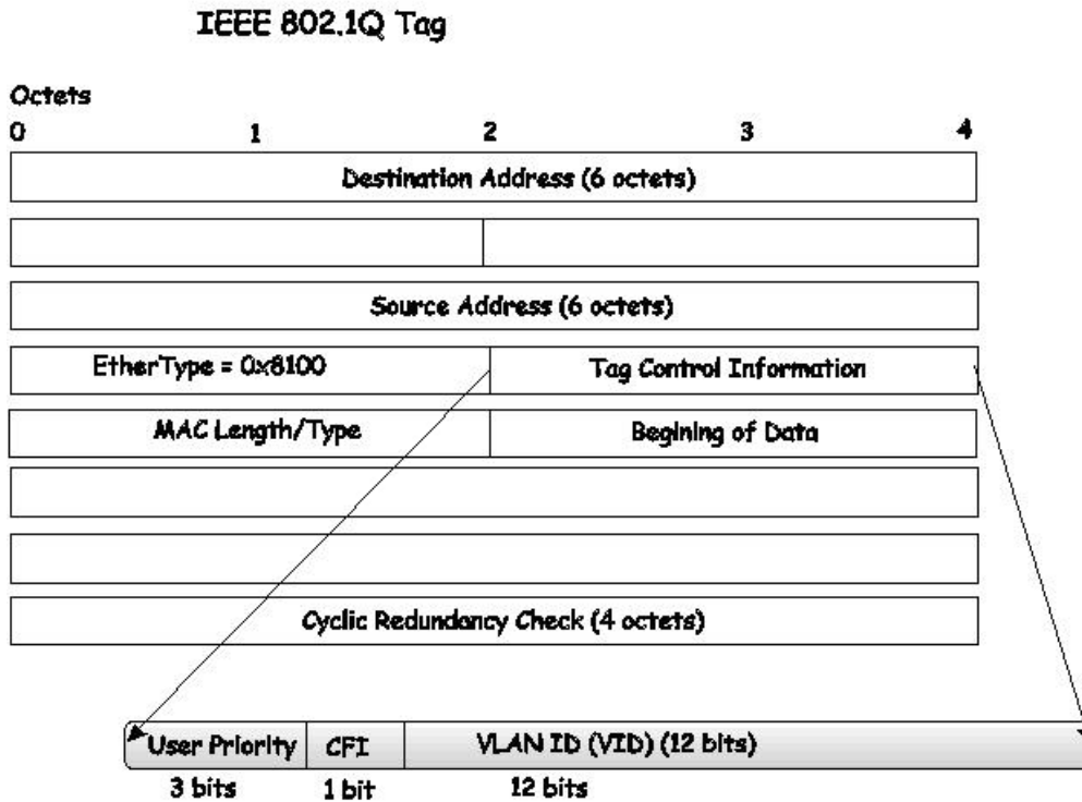
Figure 7- 2. IEEE 802.1Q Tag
