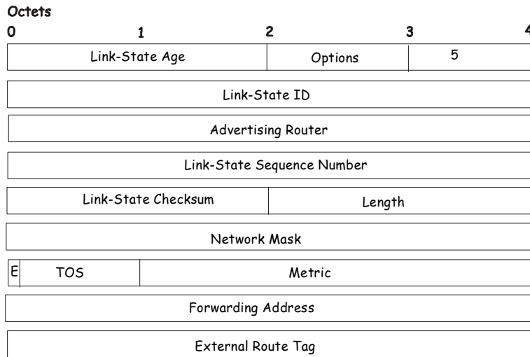
Figure 8- 41. AS External Link Advertisements
