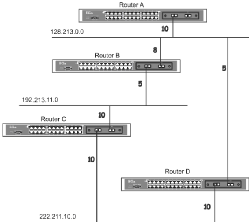
Figure 8- 28. Constructing a Shortest Path Tree
