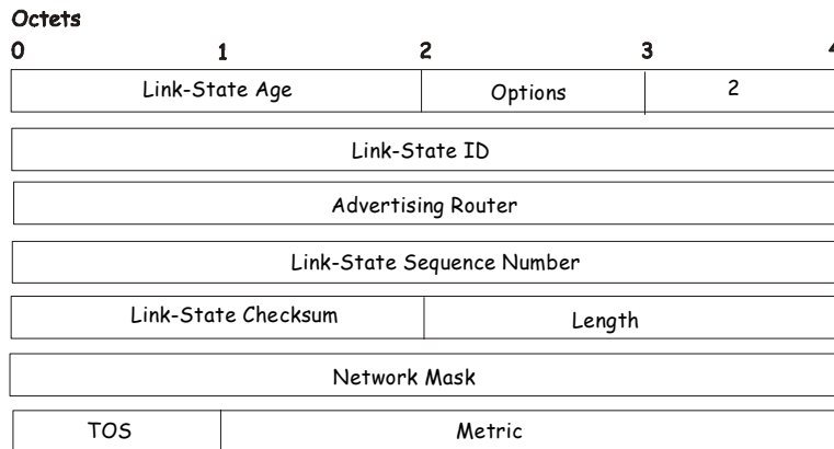
Figure 8- 40. Summary Link Advertisements
