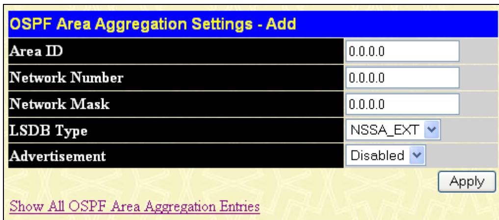
Figure 8- 52. OSPF Area Aggregation Settings – Add window
