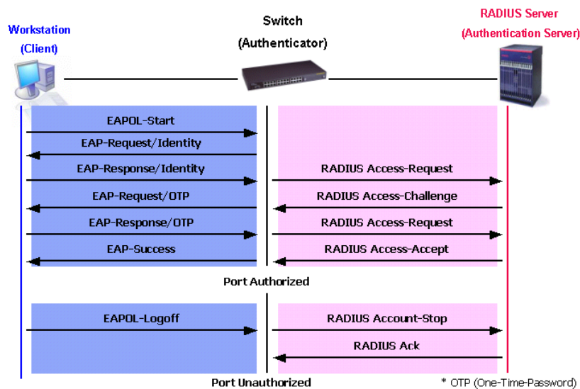
Figure 11- 14. The 802.1X Authentication Process
