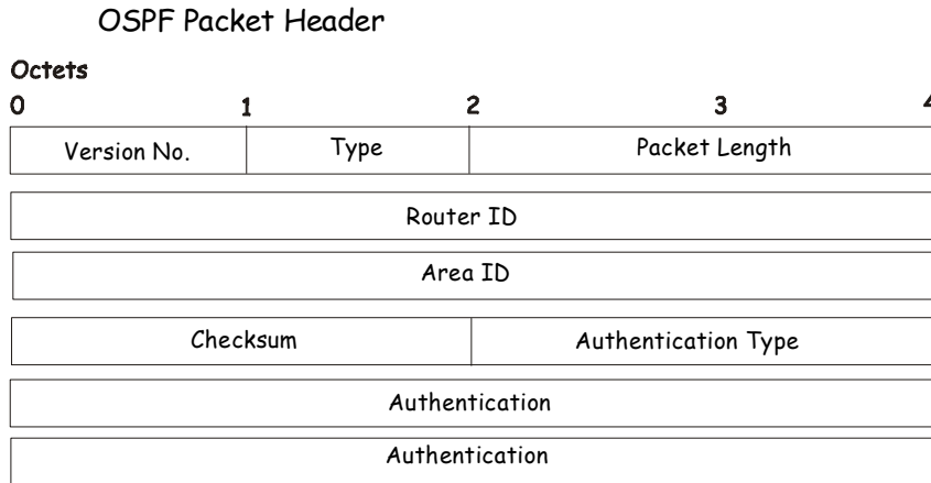
Figure 8- 31. OSPF Packet Header Format
