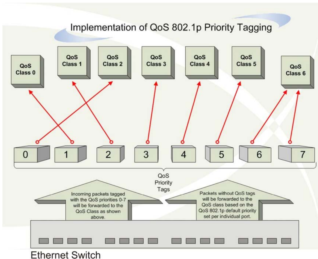
Figure 9- 1. Mapping QoS on the Switch
