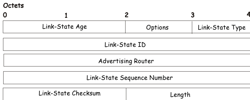
Figure 8- 37. Link State Advertisement Header
