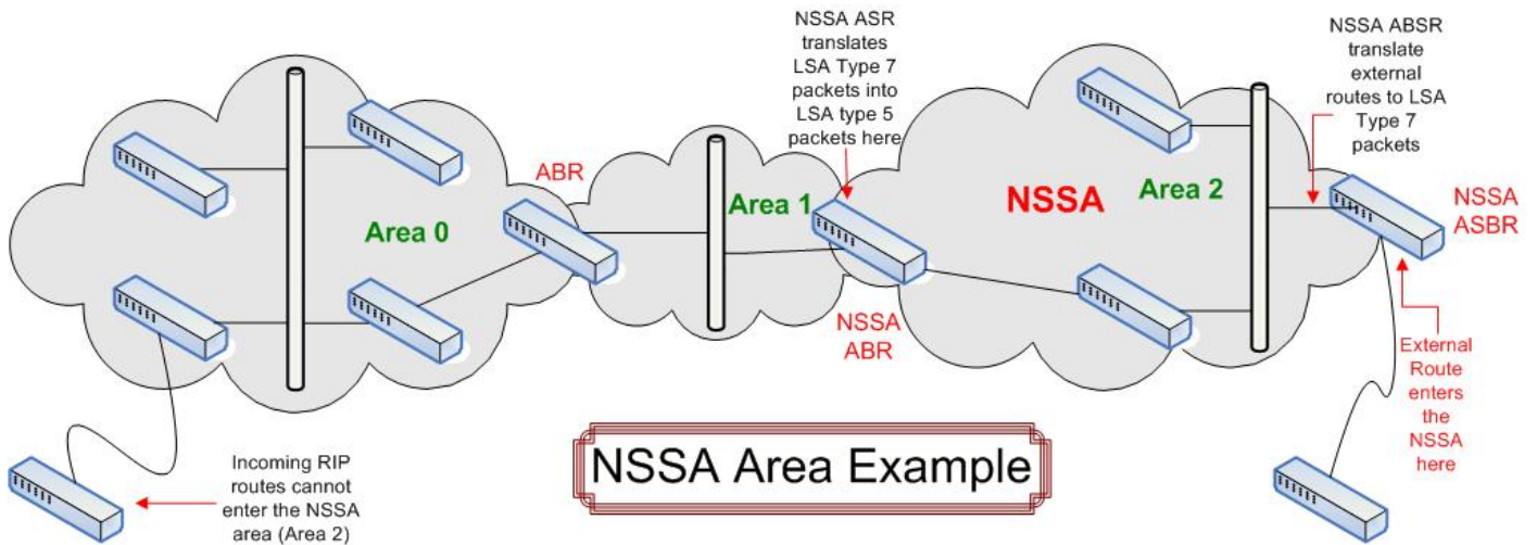
Figure 8- 42. NSSA Area example
