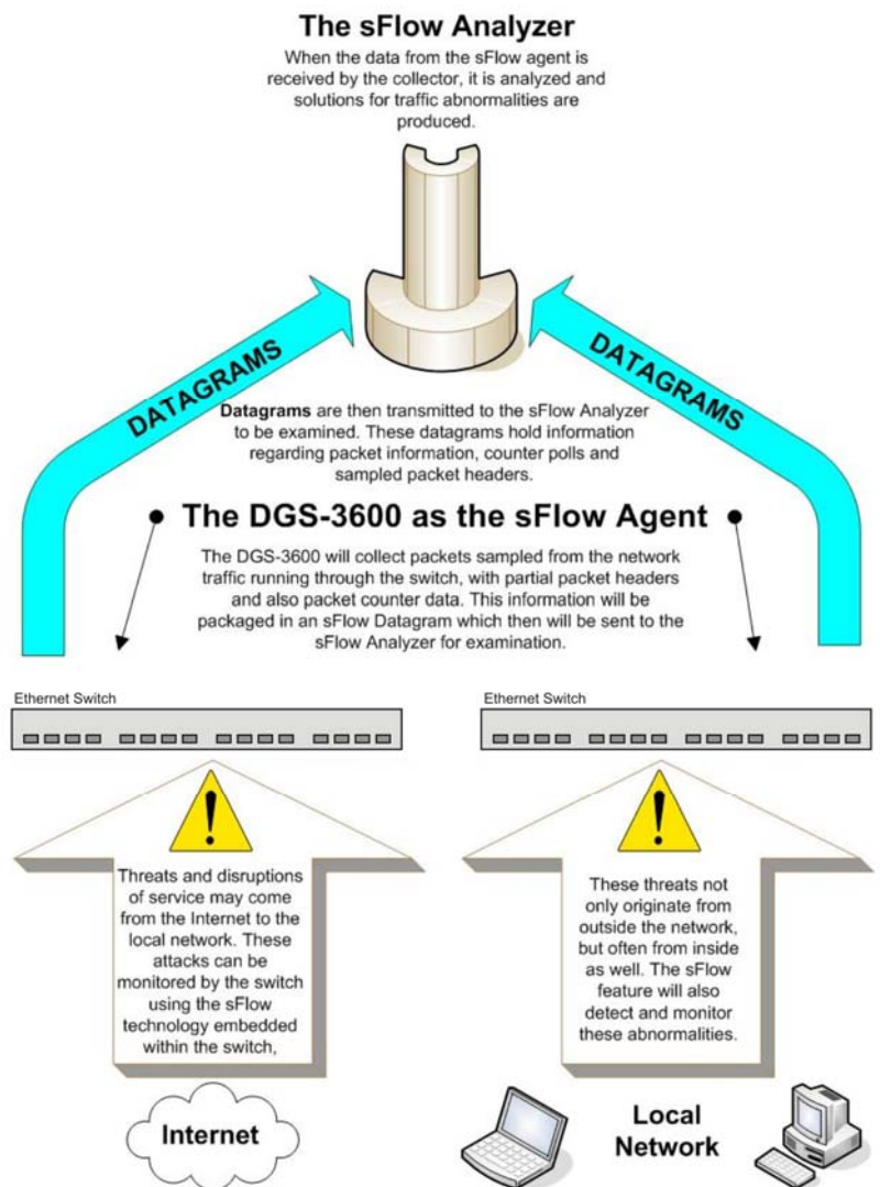
Figure 6- 52. sFlow Basic Setup
