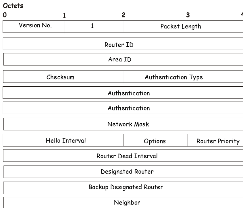
Figure 8- 32. Hello Packet
