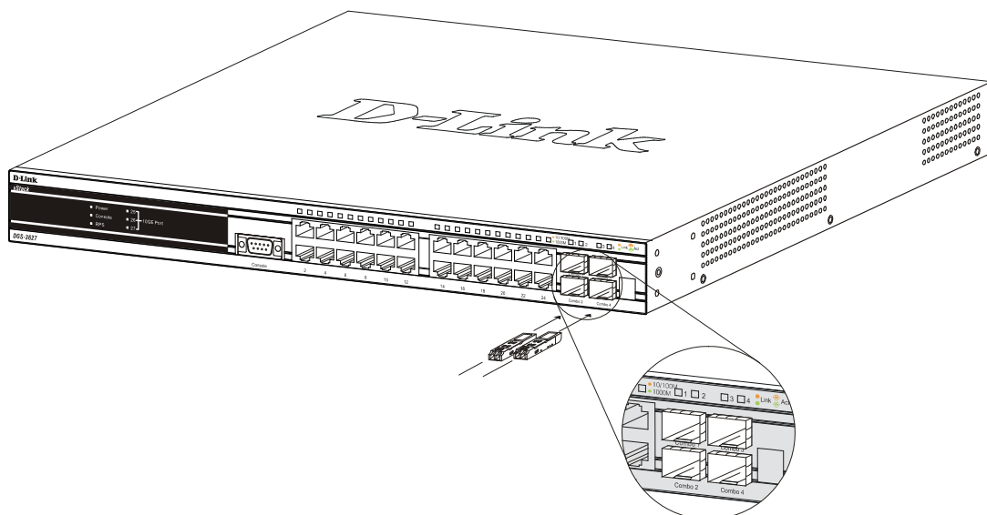
Figure 1- 25. Inserting the fiber-optic transceivers into the DGS-3600 Series switch
