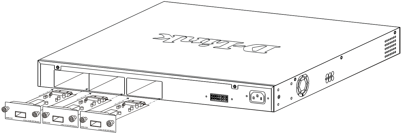
Figure 1- 23. Inserting the optional modules into the Switch.
