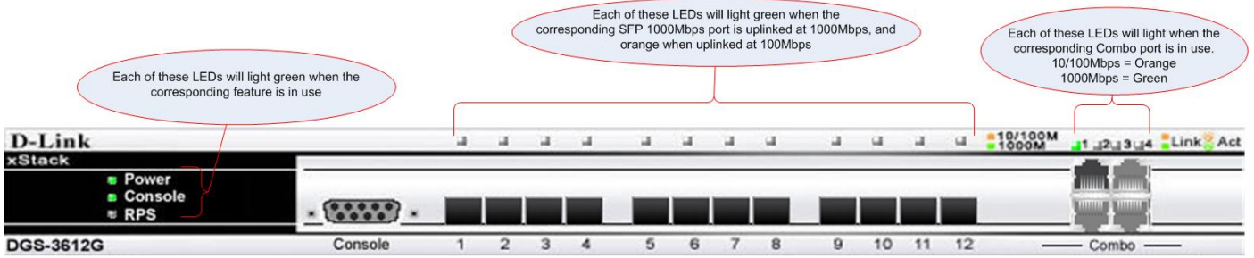
Figure 1- 6. DGS-3612G LEDs
