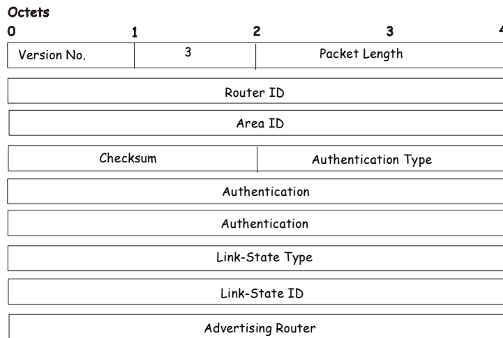
Figure 8- 34. Link-State Request Packet
