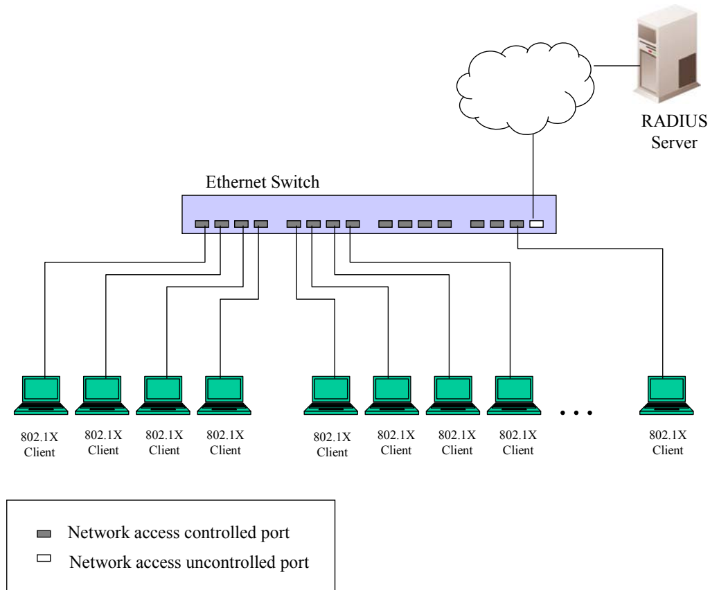
Figure 11- 15. Example of Typical Port-Based Configuration
