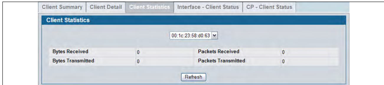
Figure 277: Client Statistics
