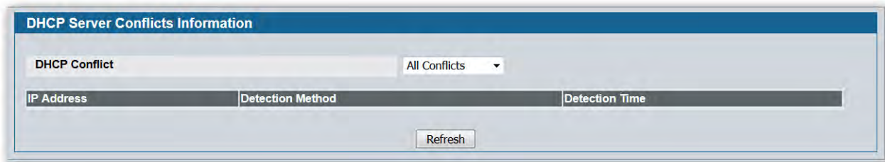
Figure 62: Conflicts Information
