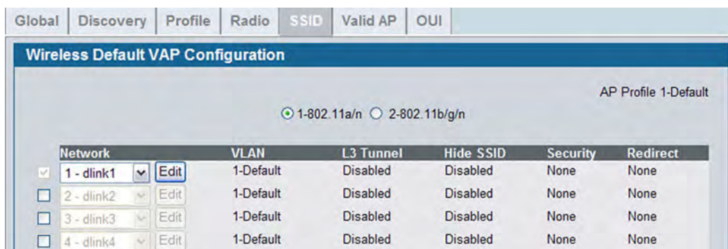
Figure 360: VAP Settings
