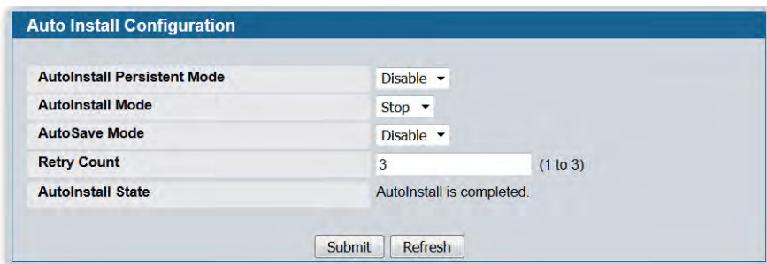
Figure 92: AutoInstall
