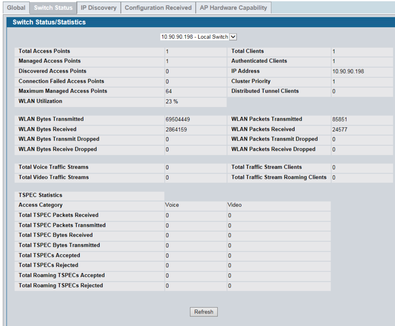
Figure 304: Switch Status/Statistics
