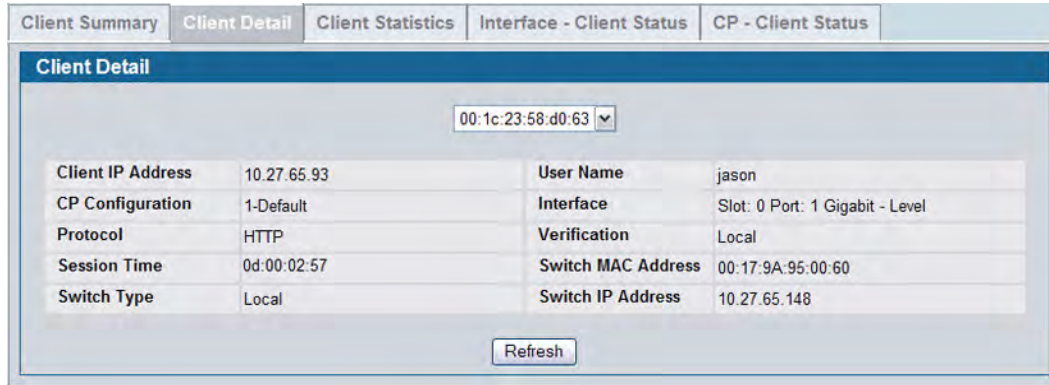
Figure 276: Client Detail
