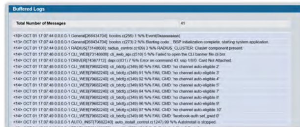
Figure 42: Buffered Log
