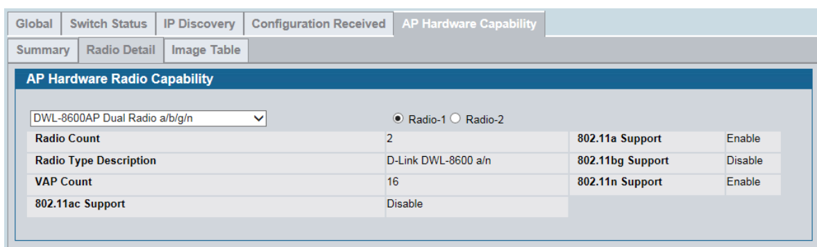
Figure 308: Radio Detail
