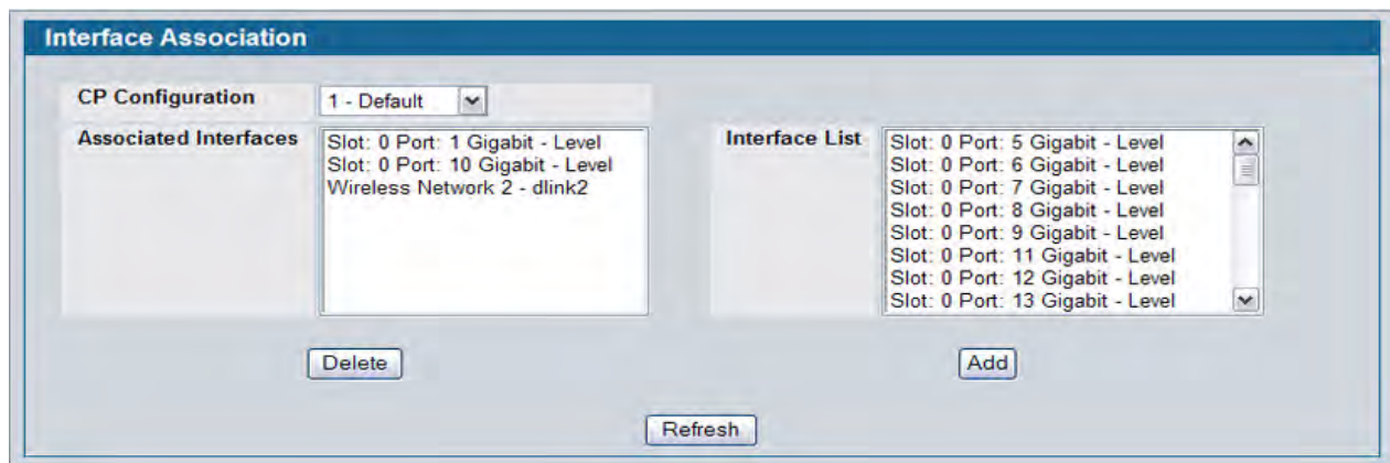
Figure 270: Interface Association
