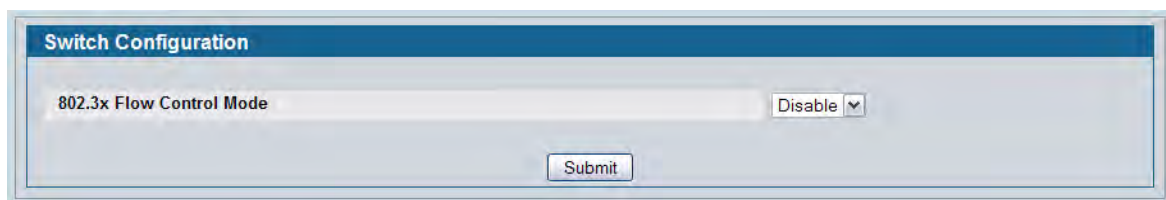
Figure 8: Switch Configuration
