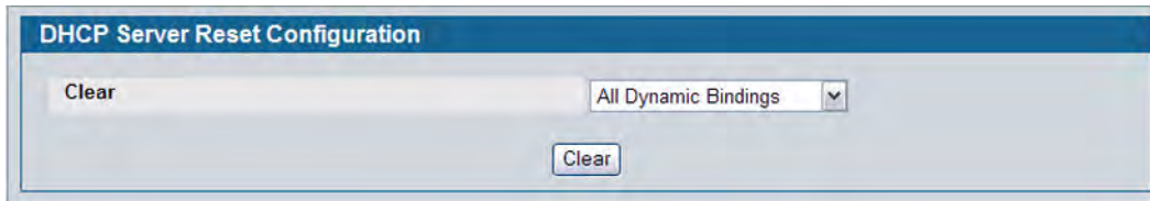
Figure 59: Reset Configuration
