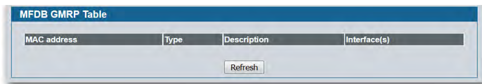
Figure 144: GMRP Table
