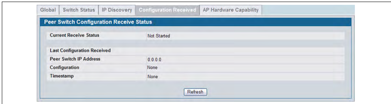
Figure 306: Configuration Received
