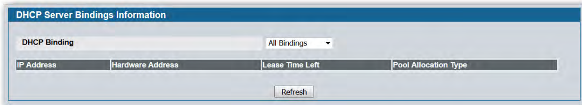
Figure 60: Bindings Information
