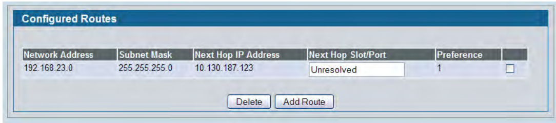
Figure 204: Configured Routes
