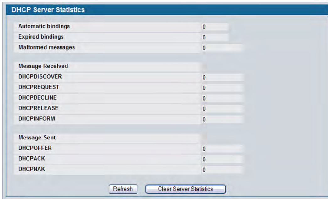
Figure 61: Server Statistics
