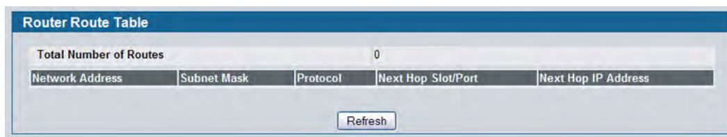
Figure 202: Route Table
