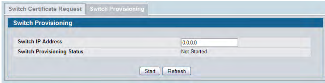
Figure 400: Switch Provisioning
