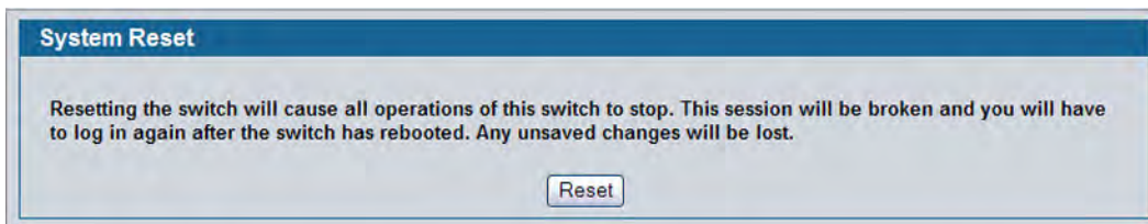
Figure 84: System Reset
