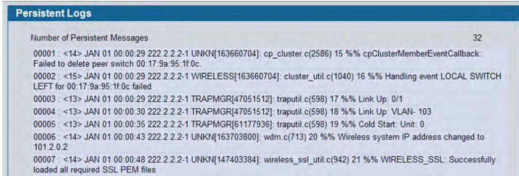
Figure 49: Persistent Log
